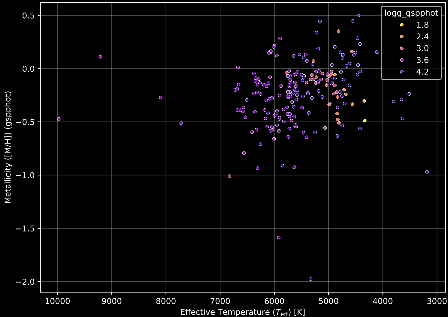
APOGEE DR17 Field: [142-47_MGA] Stellar Population Parameters (n= 203)
