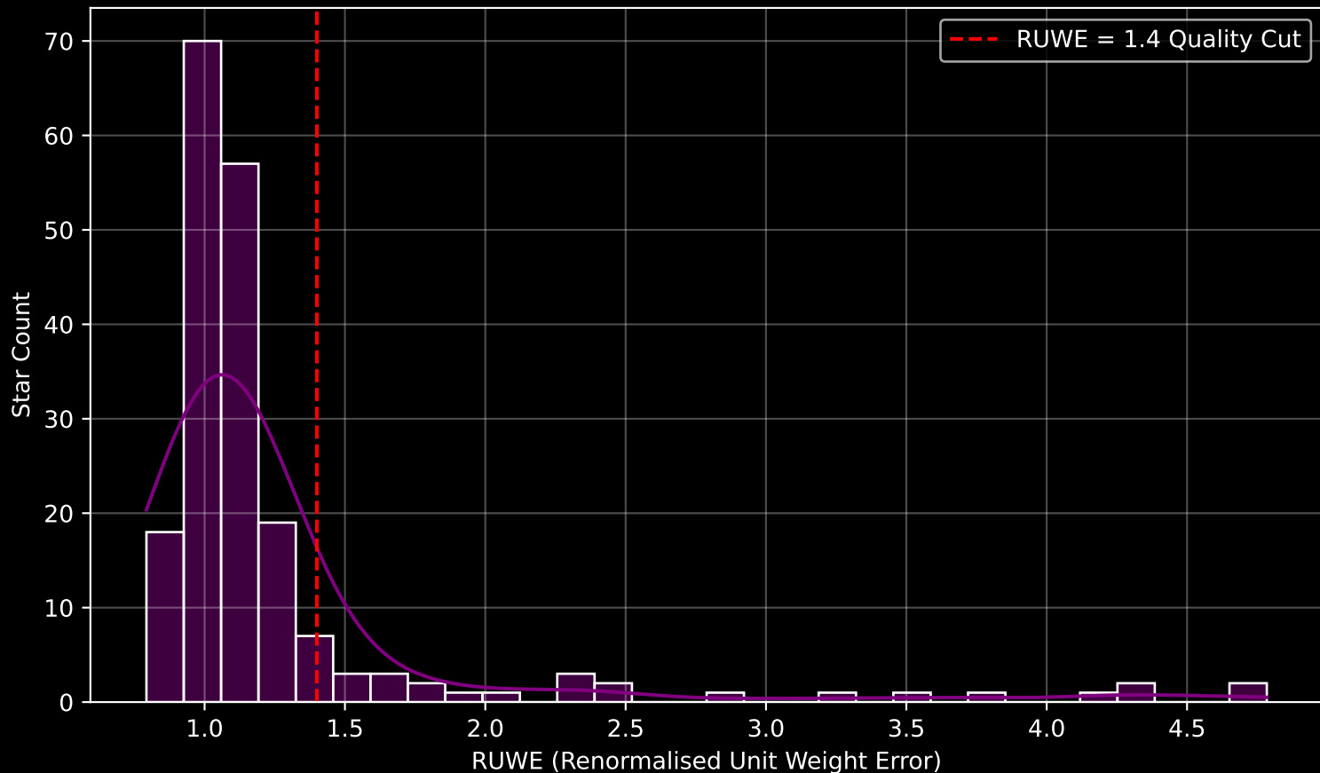
GAPOGEE DR17 Field [142-47_MGA] RUWE Distribution (n= 195)
