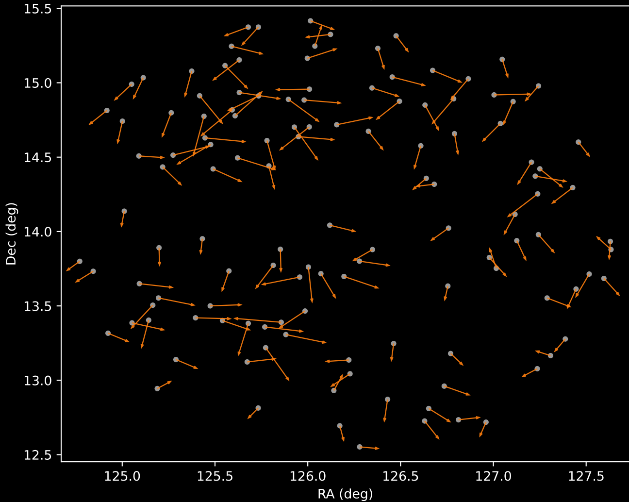
APOGEE DR17 Cluster 2 Proper Motion Vectors (n=125)
