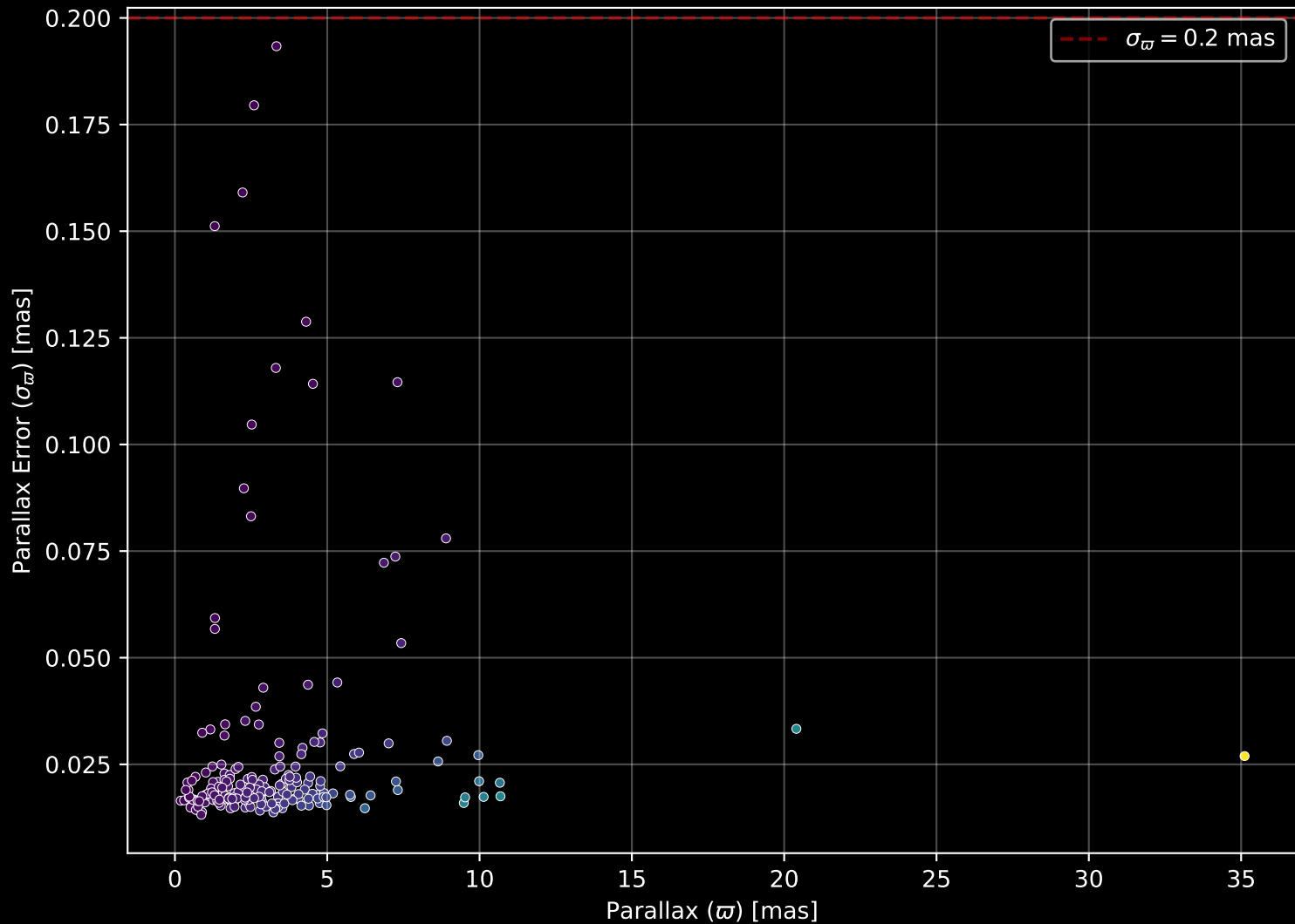
APOGEE DR17 Field: [142-47_MGA] Parallax Quality (n= 203)
