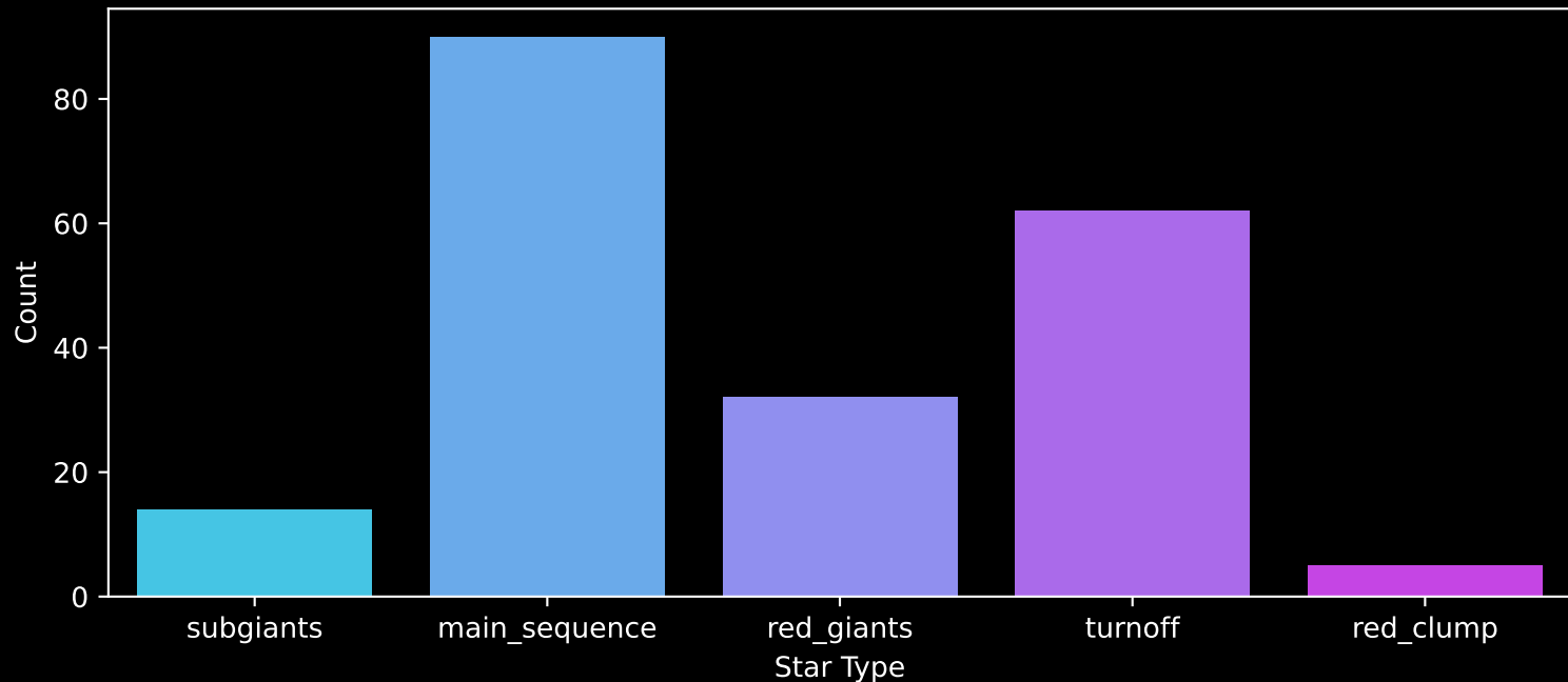
APOGEE DR17 Field: [142-47_MGA] Count plot of Star Type
