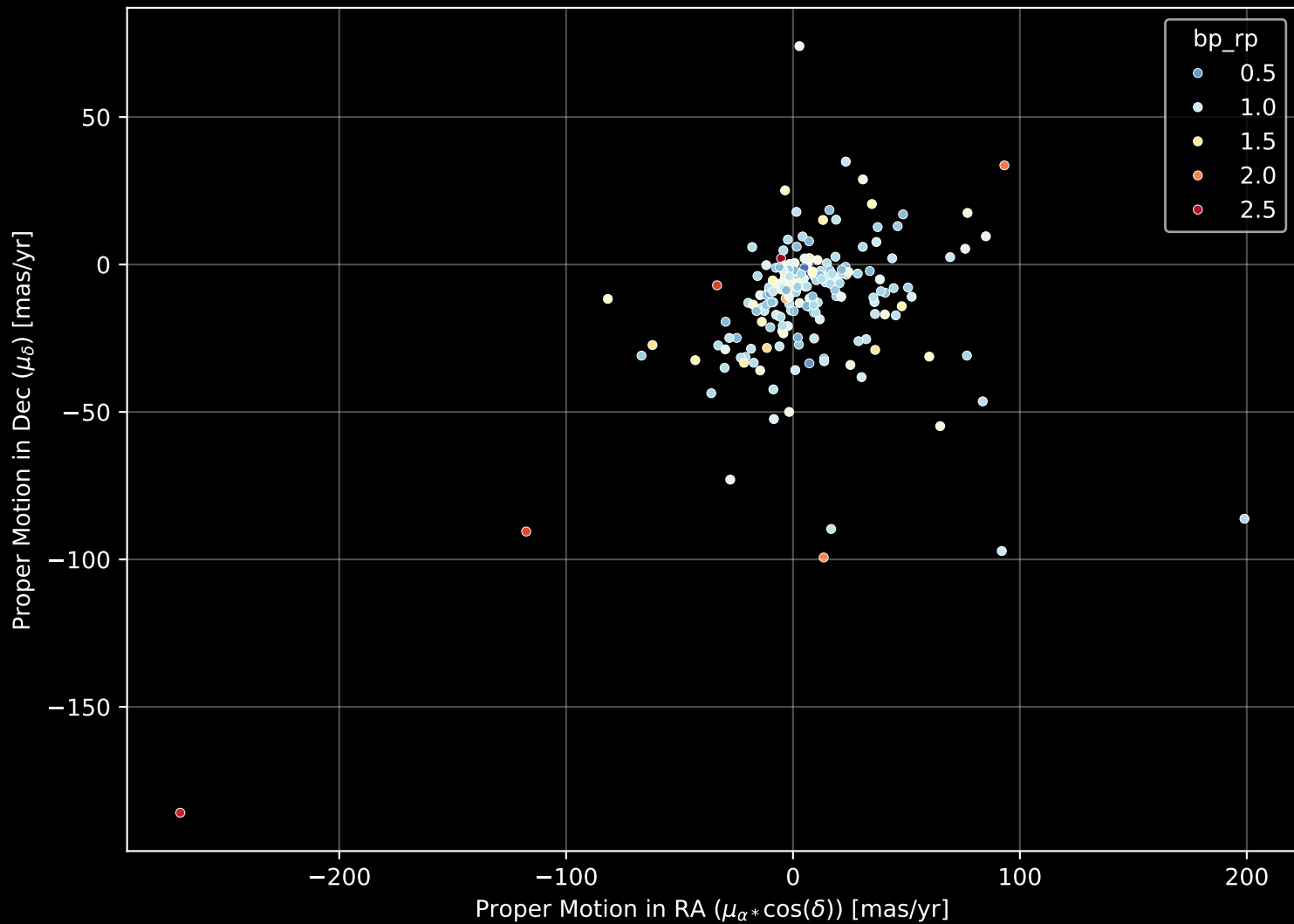
APOGEE DR17 Field: [142-47_MGA] Proper Motion Diagram (n= 203)
