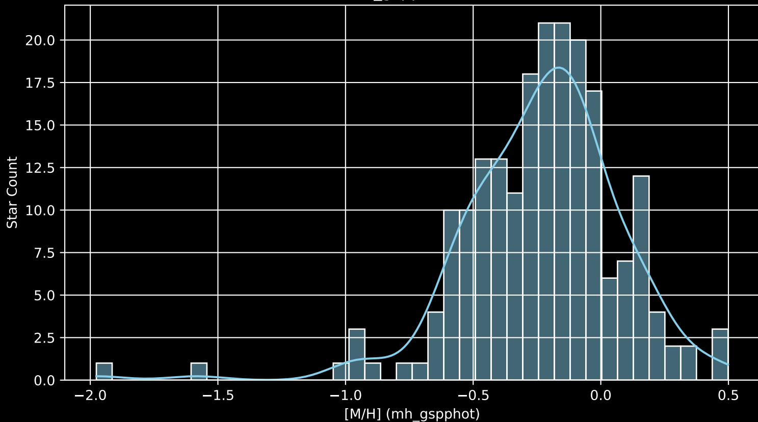
APOGEE DR17 Field: [142-47_MGA [M/H] (mh_gspphot) (n= 203)
